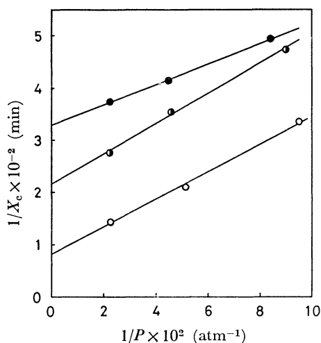
Fig. 5. Relation between 1/P and 1/X_c . Temp: ○ 120, ◐ 108, ● 100 °C. Other conditions were shown in Table 2.
